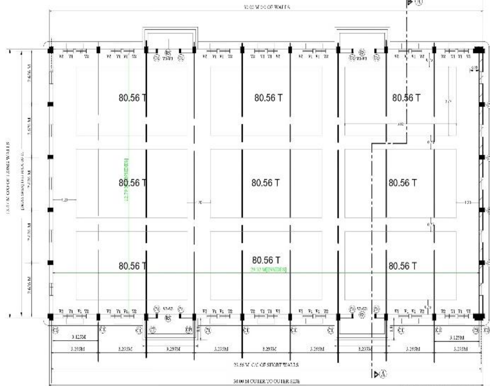
PLAN FOR 725 MT. WAREHOUSE UNIT NO. I, II
